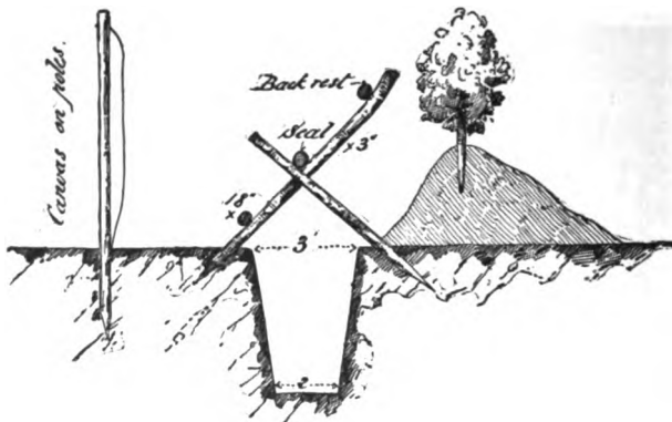
FIG. 223.—Field Sink.
