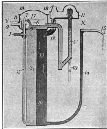
FIG. 207.—Diagrammatic Sketch of Forbes Water Sterilizer—A.my Type.
