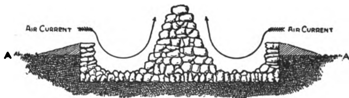
FIG. 229.—Crematory—Vertical Section. A A, Ground level.
