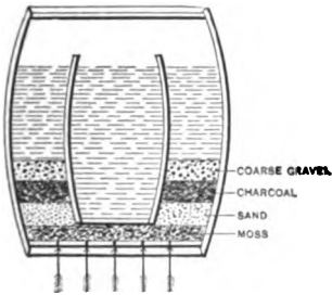
FIG. 213. — Improvised Filter.
